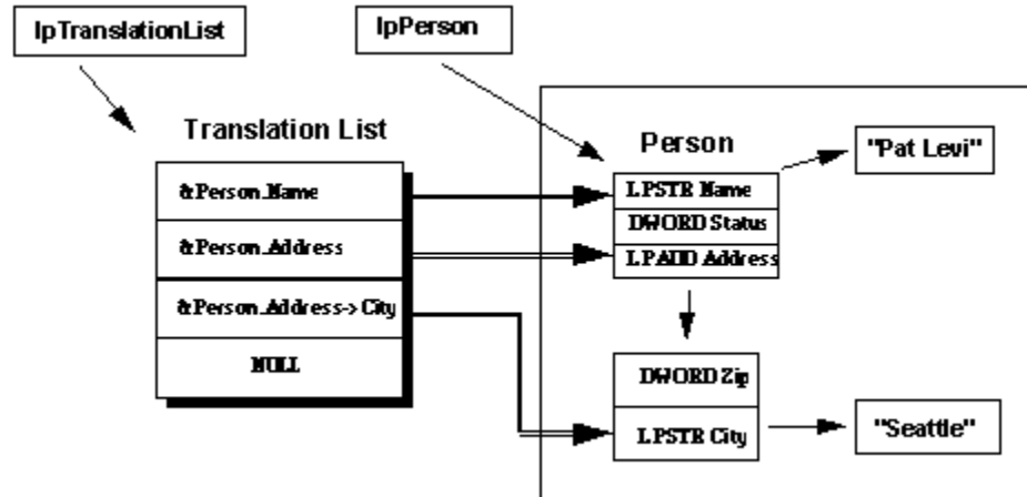
Figure 4. Translation List
