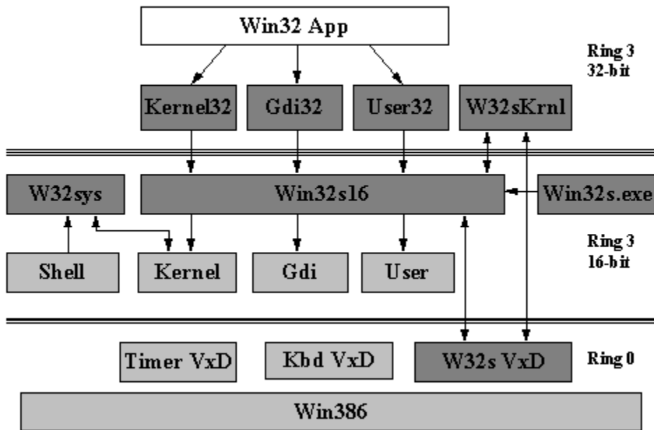
Figure 1. Win32s Architecture.
